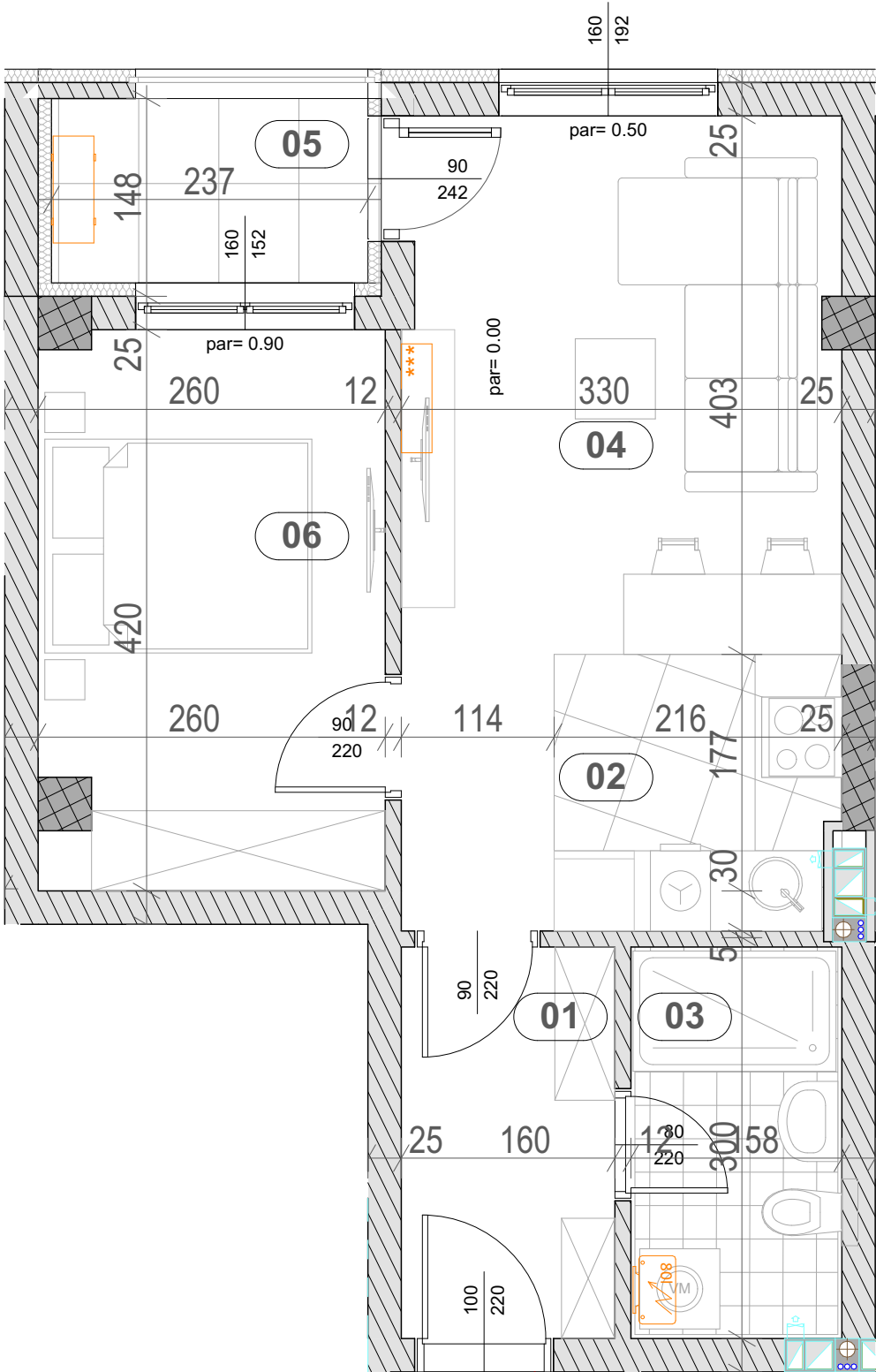
S19 (41.80m 2 )
